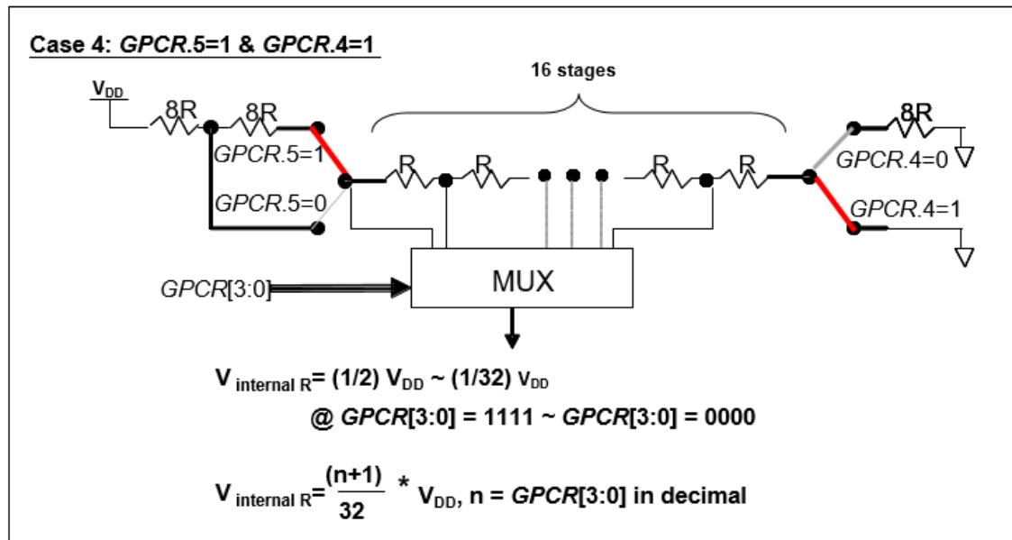
Fig. 26: V_{internal\ R} hardware connection if GPCR.5=1 and GPCR.4=1
