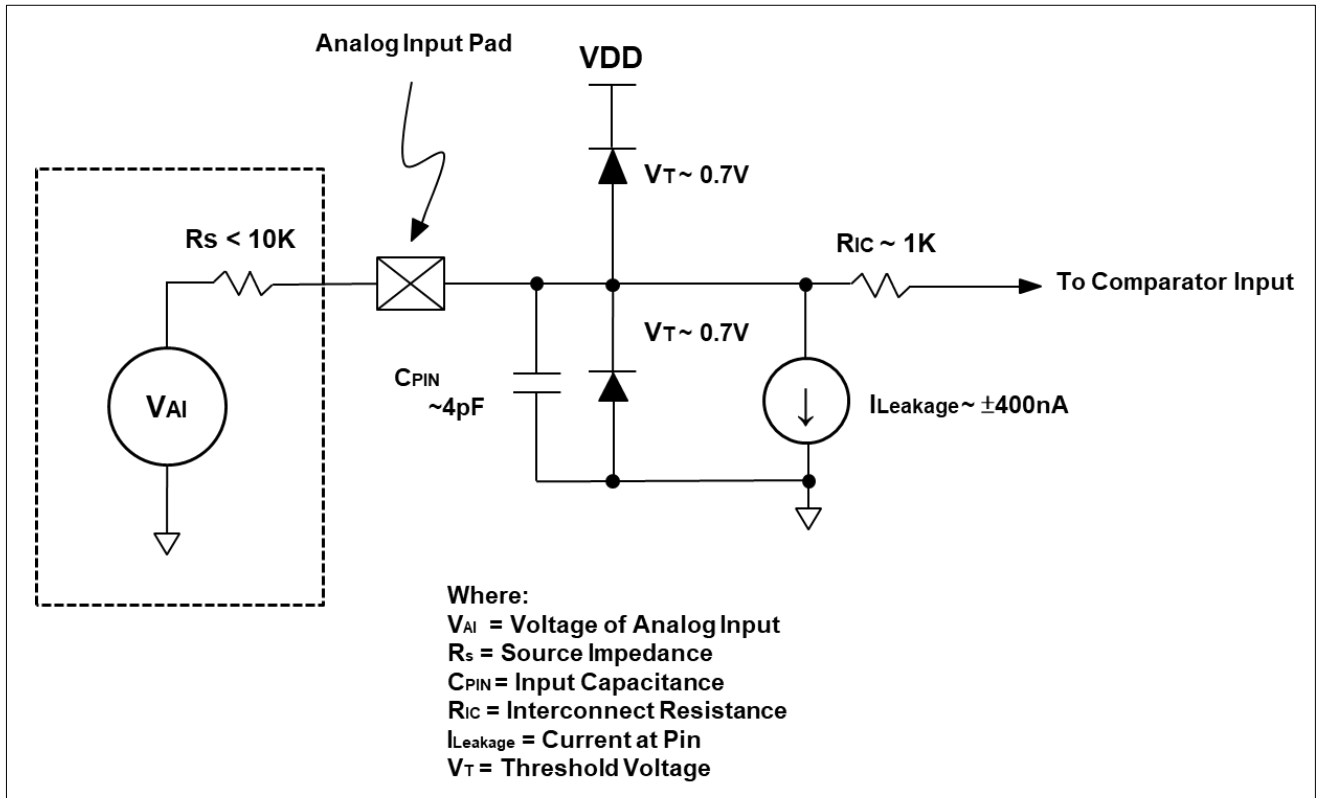
Fig.22: Analog Input Model of General-Purpose Comparator
