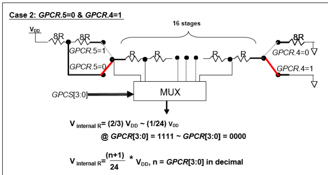
Fig. 24: V_{\text{internal R}} hardware connection if GPCR.5=0 and GPCR.4=1
