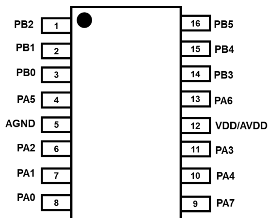
MF324-S16A: SOP16(150mil)
