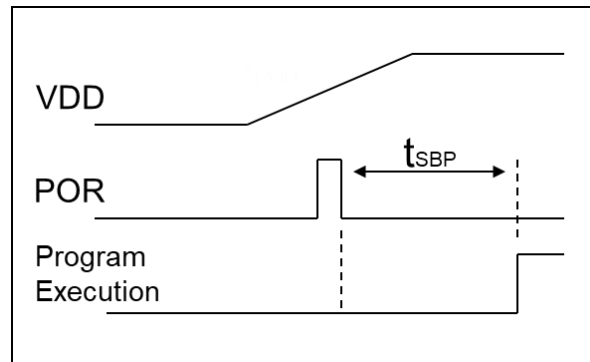
Fig.8: Power-On Sequence
